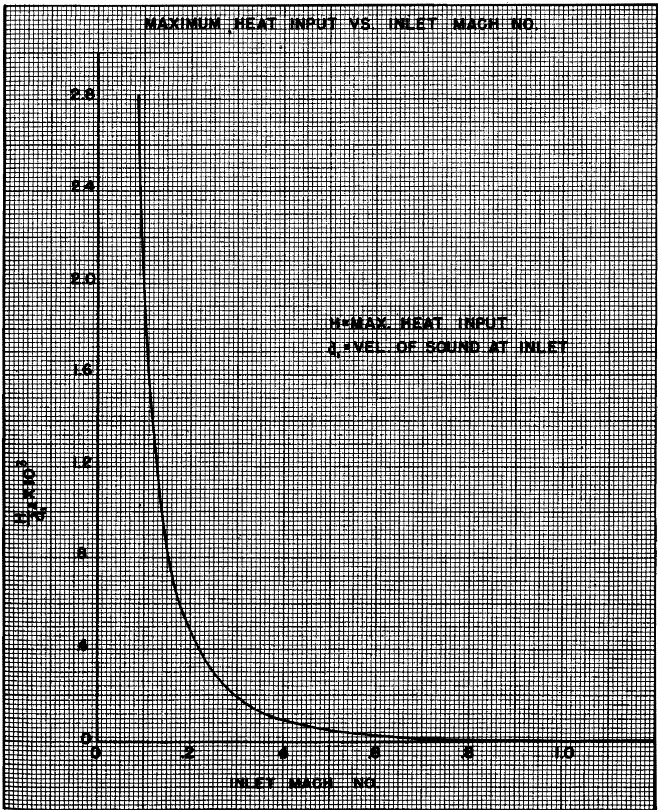
Figure 17 — Combustion Chamber Characteristics (Maximum Heat Input vs. Inlet Mach Number)
