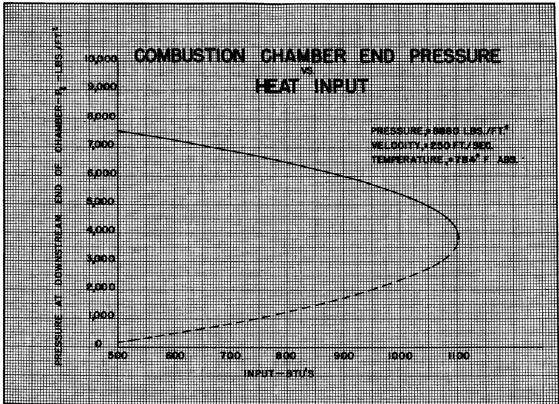
Figure 18 — Combustion Chamber End Pressure vs. Heat Input
