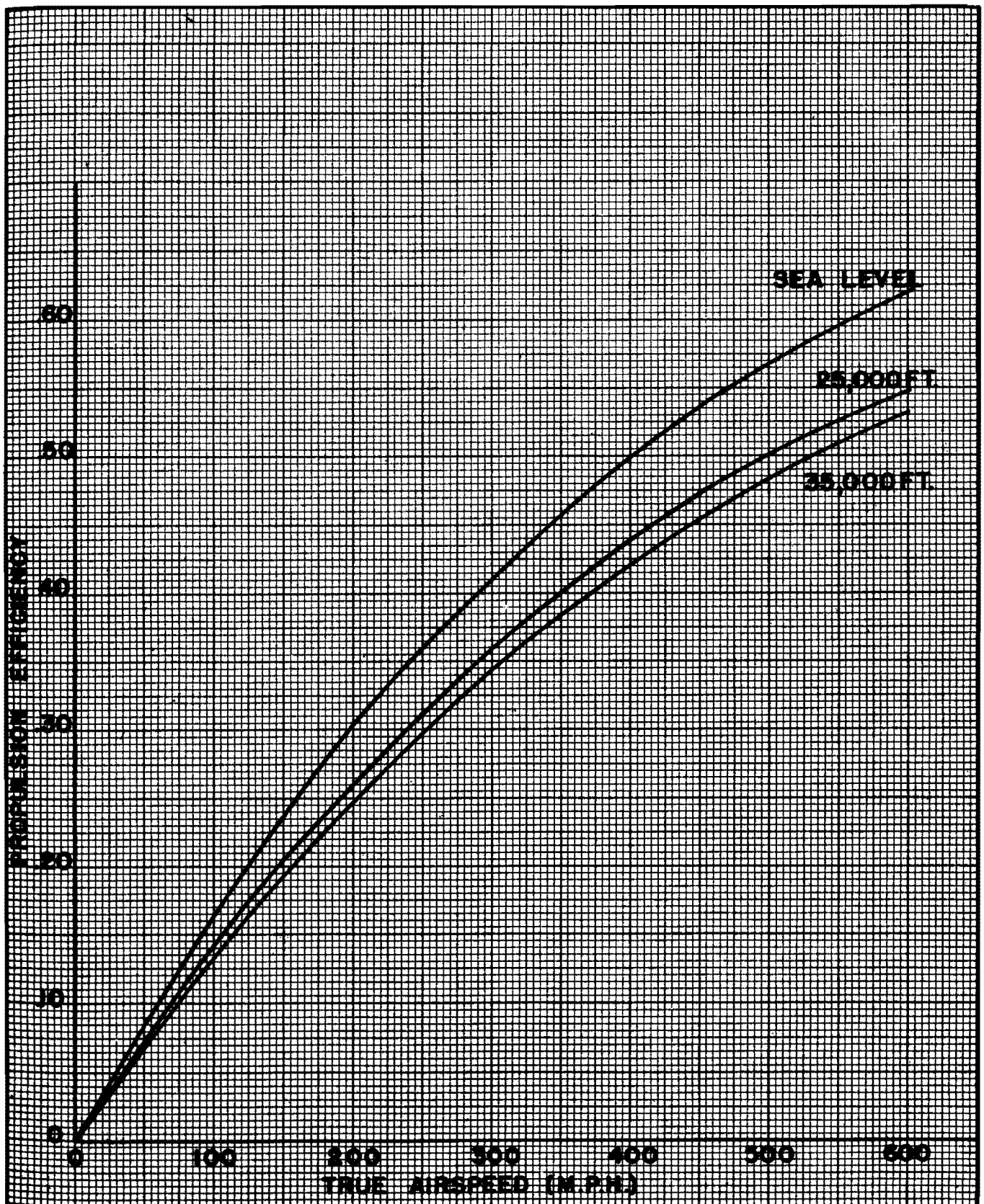
Figure 13 — Type I-40 Turbojet (11,500 RPM)
