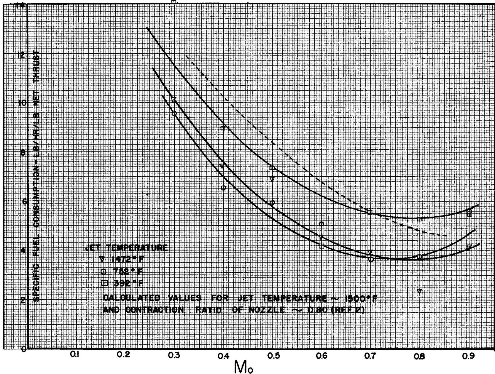
Figure 8 — Calculated Values for Jet Temperature — 1500°F and Contraction Ratio of Nozzle — 0.80 (Ref. 2)
