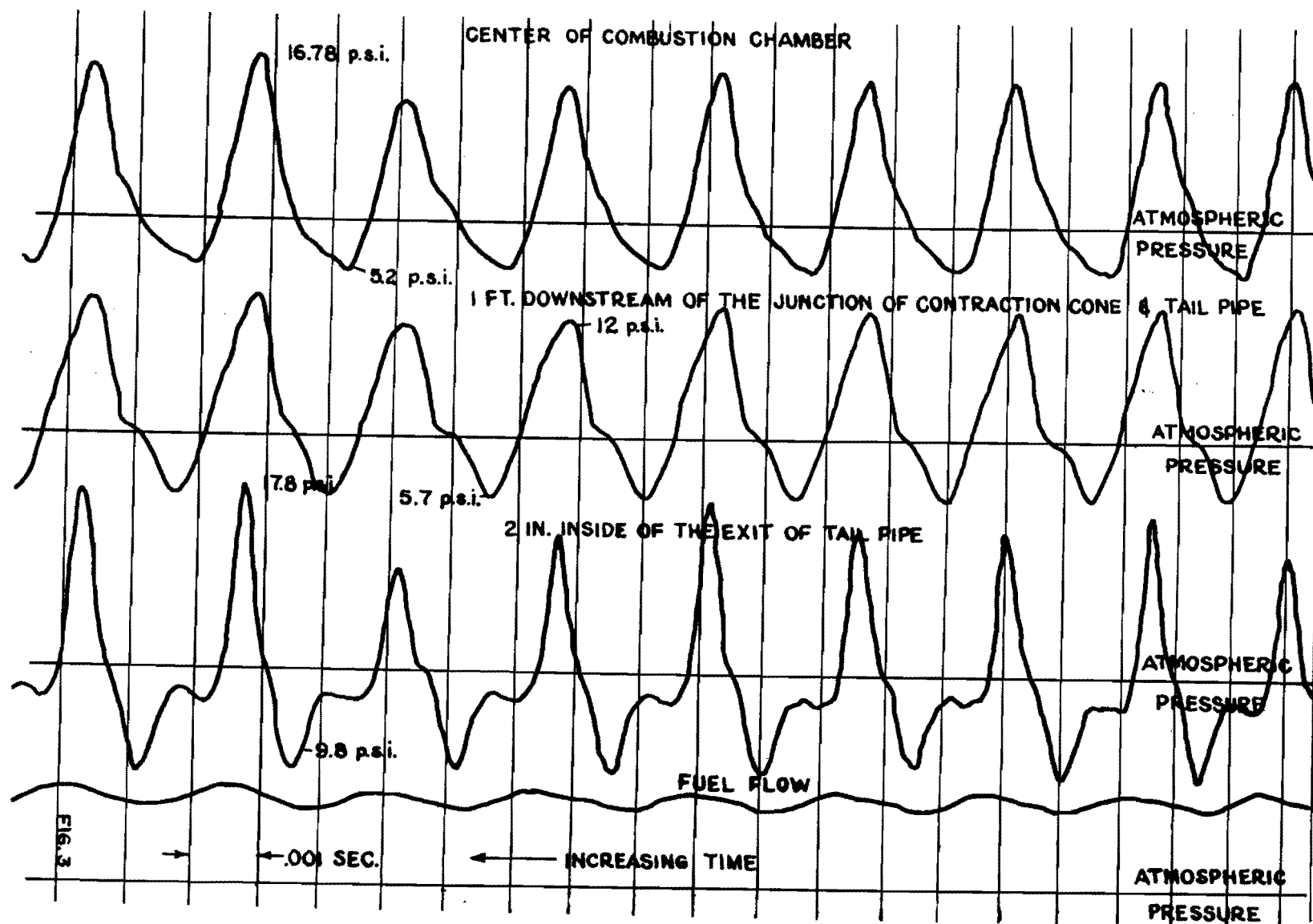
Figure 3 — 31 in. H_2O Ram and 37 psi Injection Nozzle Pressure. Pressures are Wall Statics
