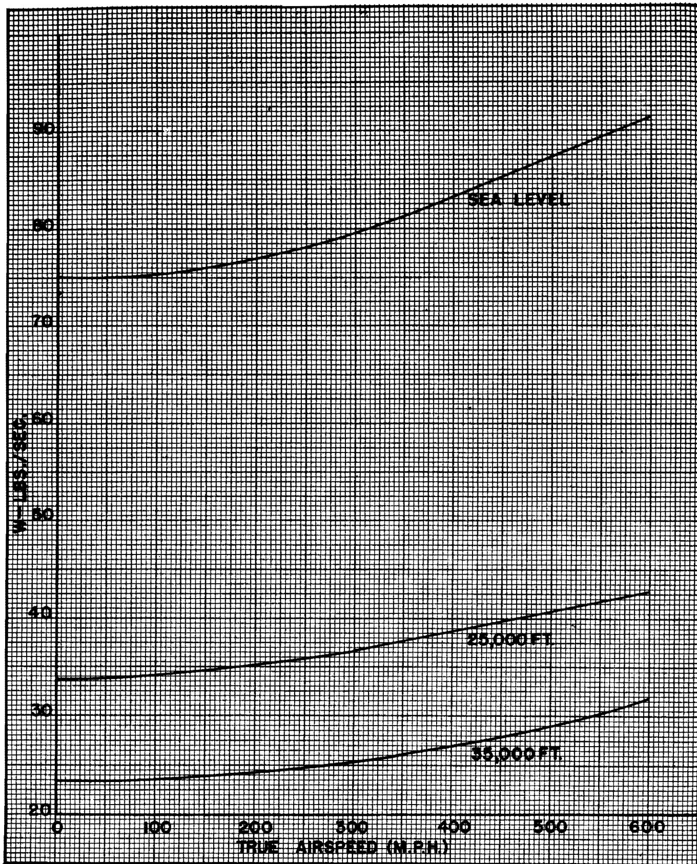
Figure 12 — Type I-40 Turbojet (11,500 RPM)
