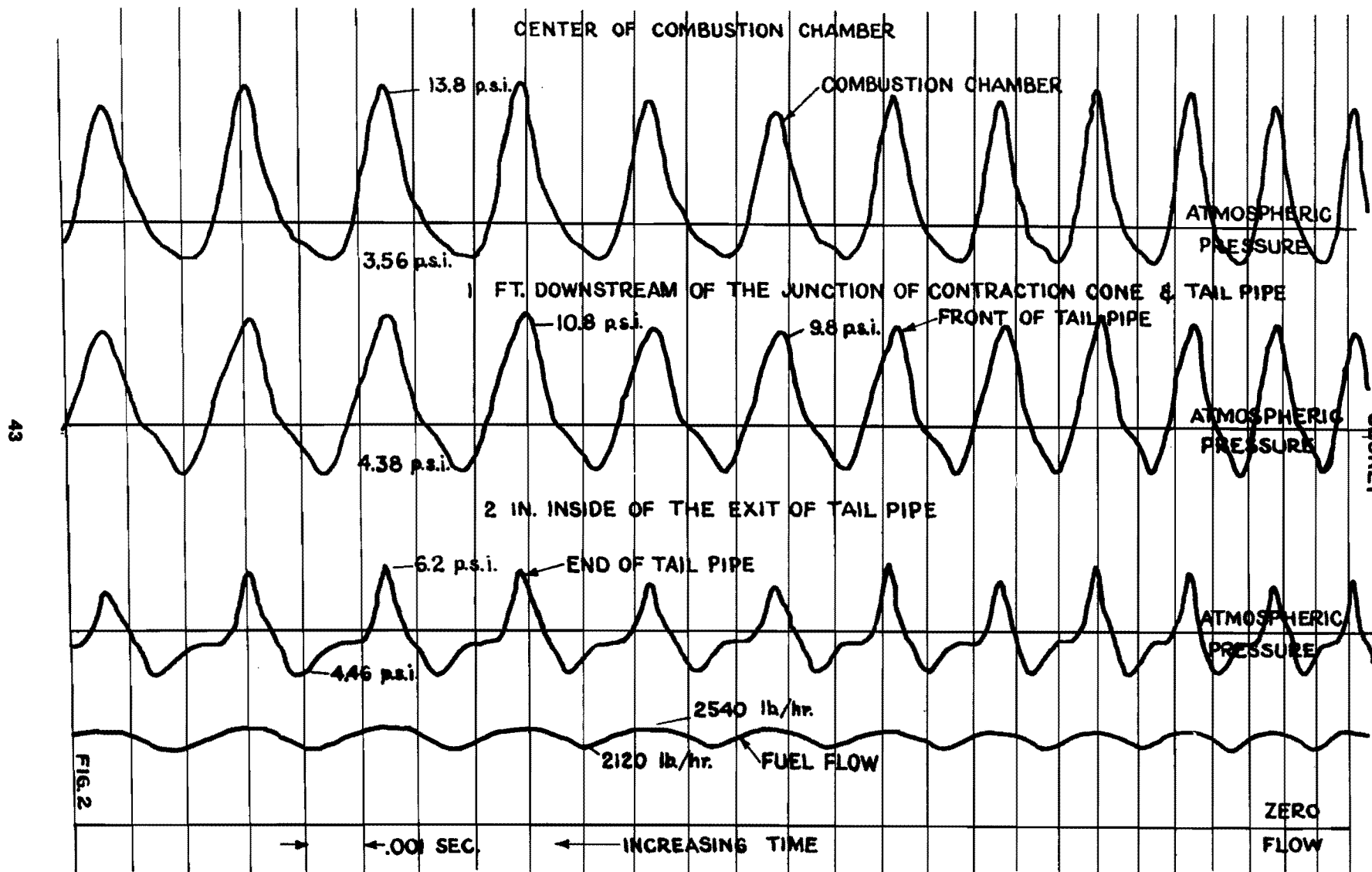
Figure 2 — 10 in. H_2O Ram and 23 p.s.i. Injection Nozzle Pressure. Pressures are Wall Statics
