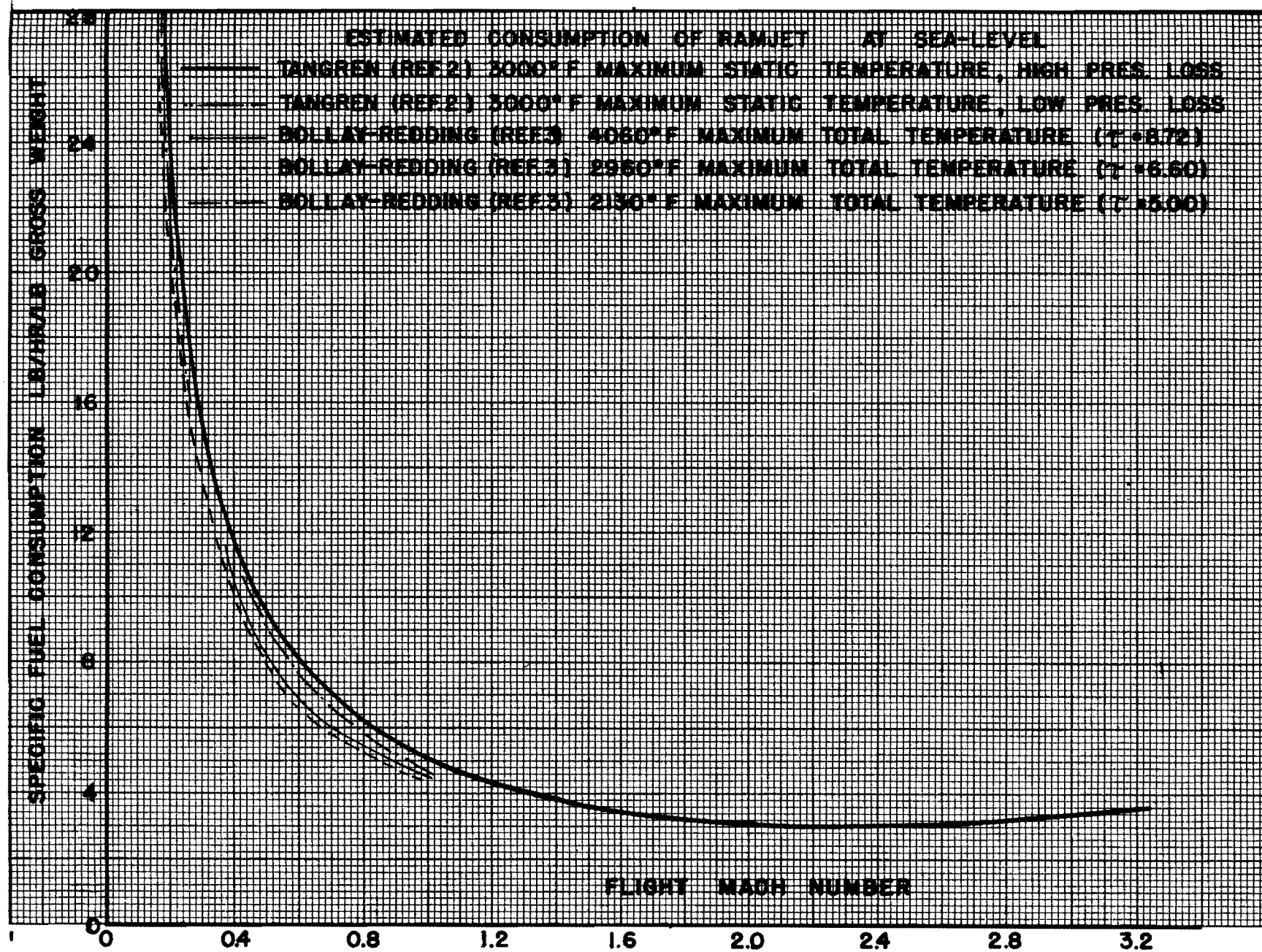
Figure 4 — Estimated Consumption of Ramjet at Sea Level
