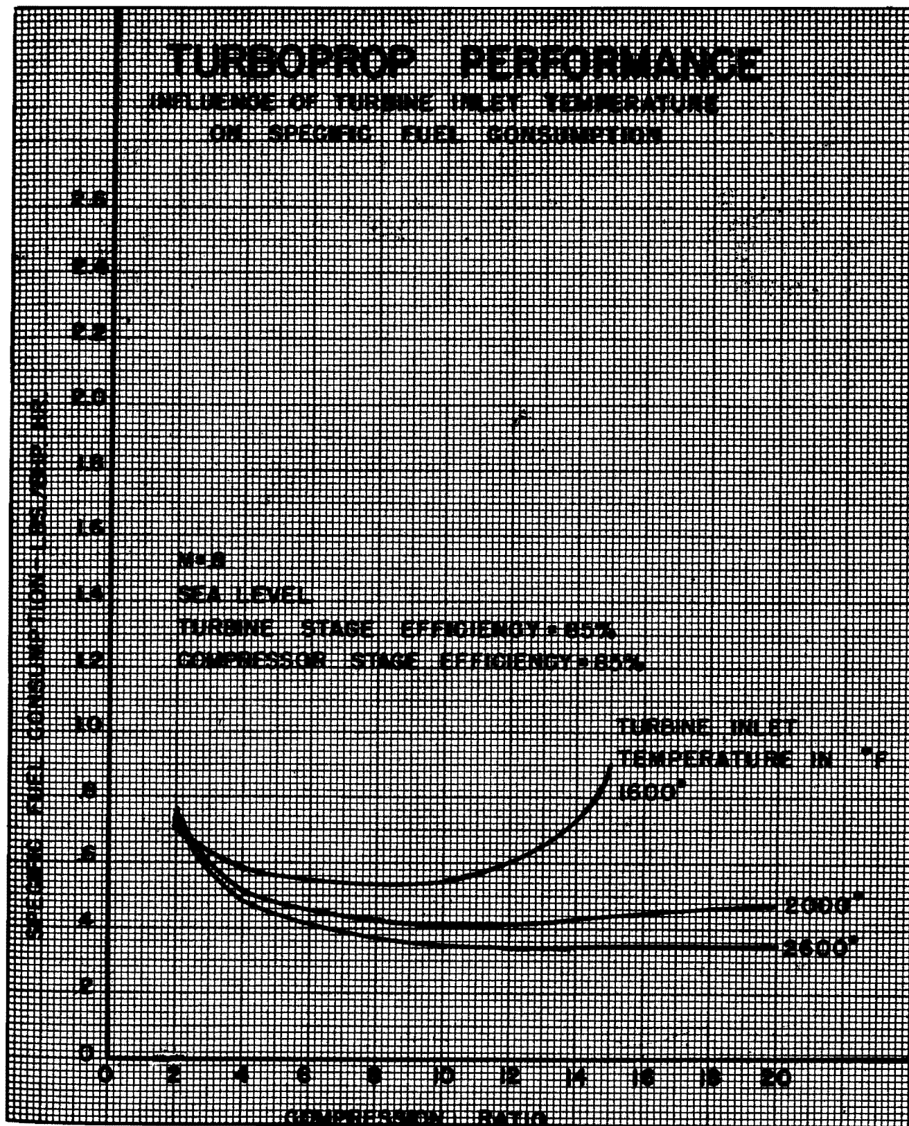
Figure 3 — Turboprop Performance (Influence of Turbine-Inlet Temperature on Specific Fuel Consumption)
