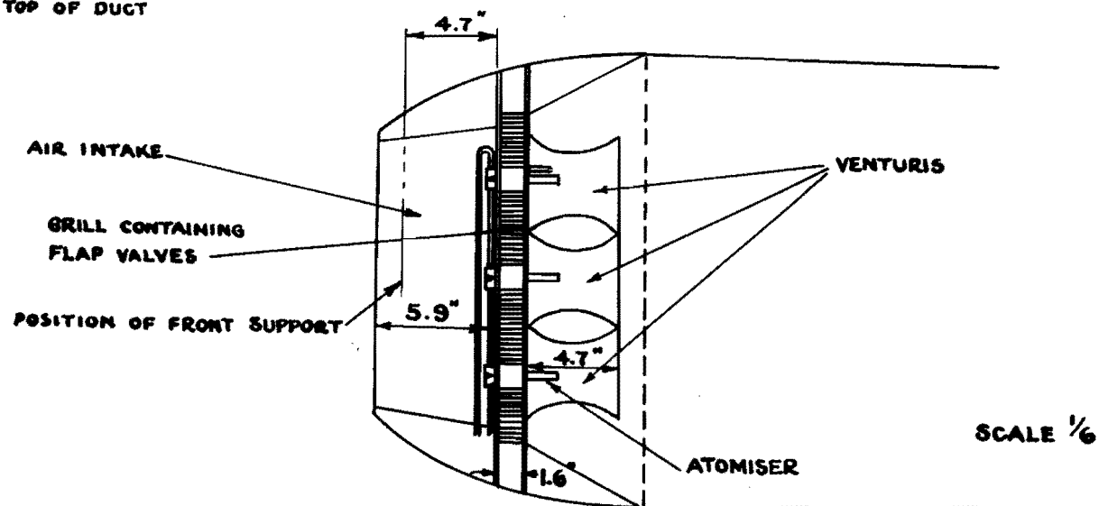
Figure 1 — German Aeropulse — General Arrangement of Duct
