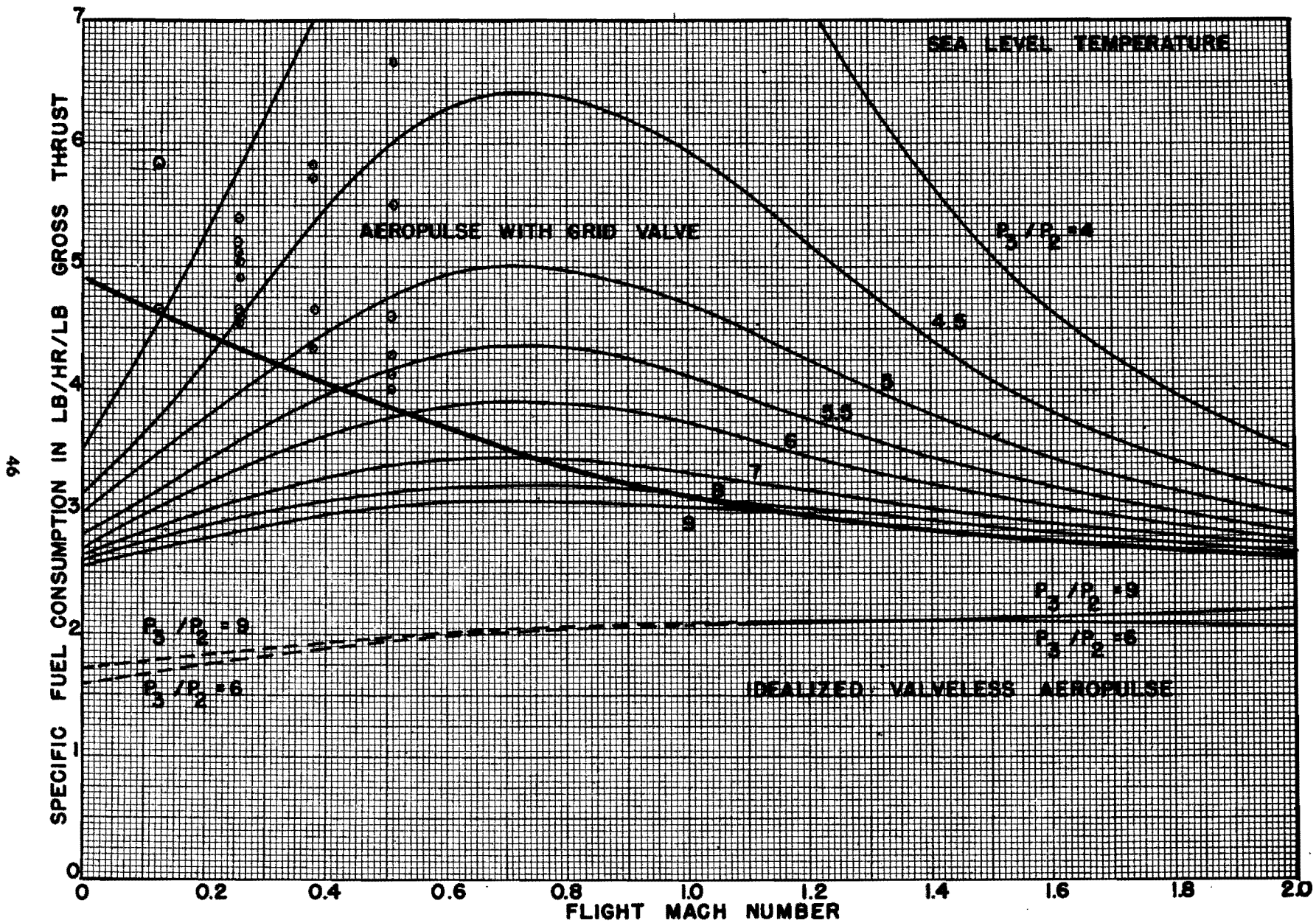
Figure 4 — Test results on the German Aeropulse
