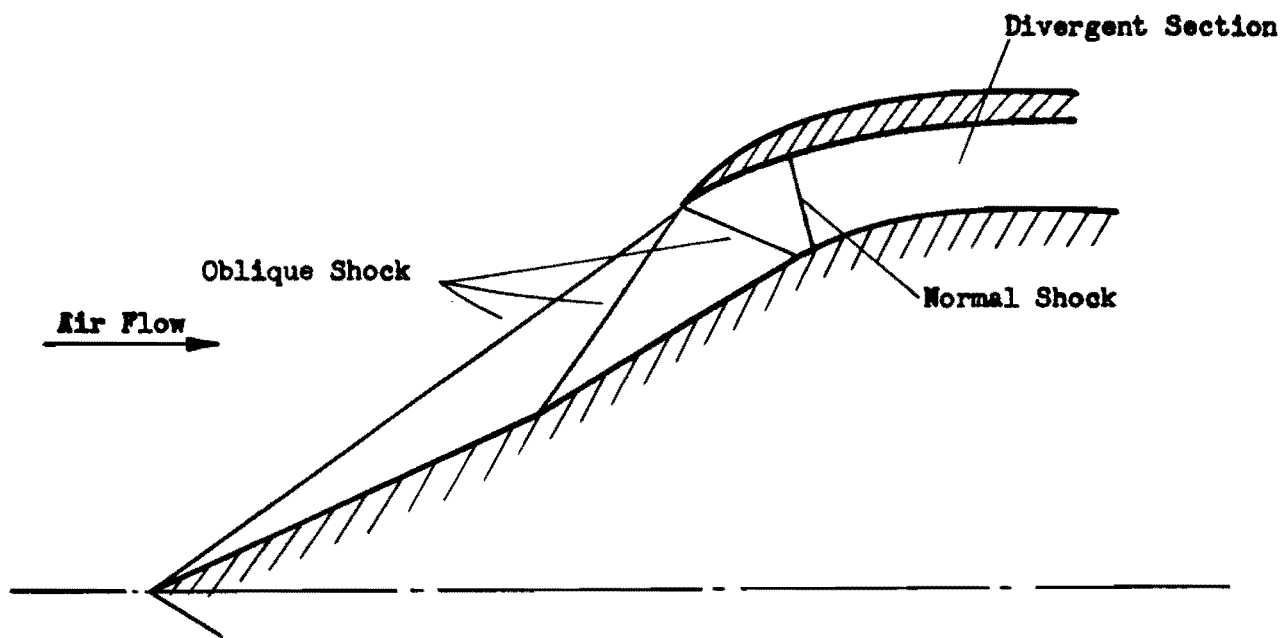
Figure 3 — Oswatitsch Diffuser
