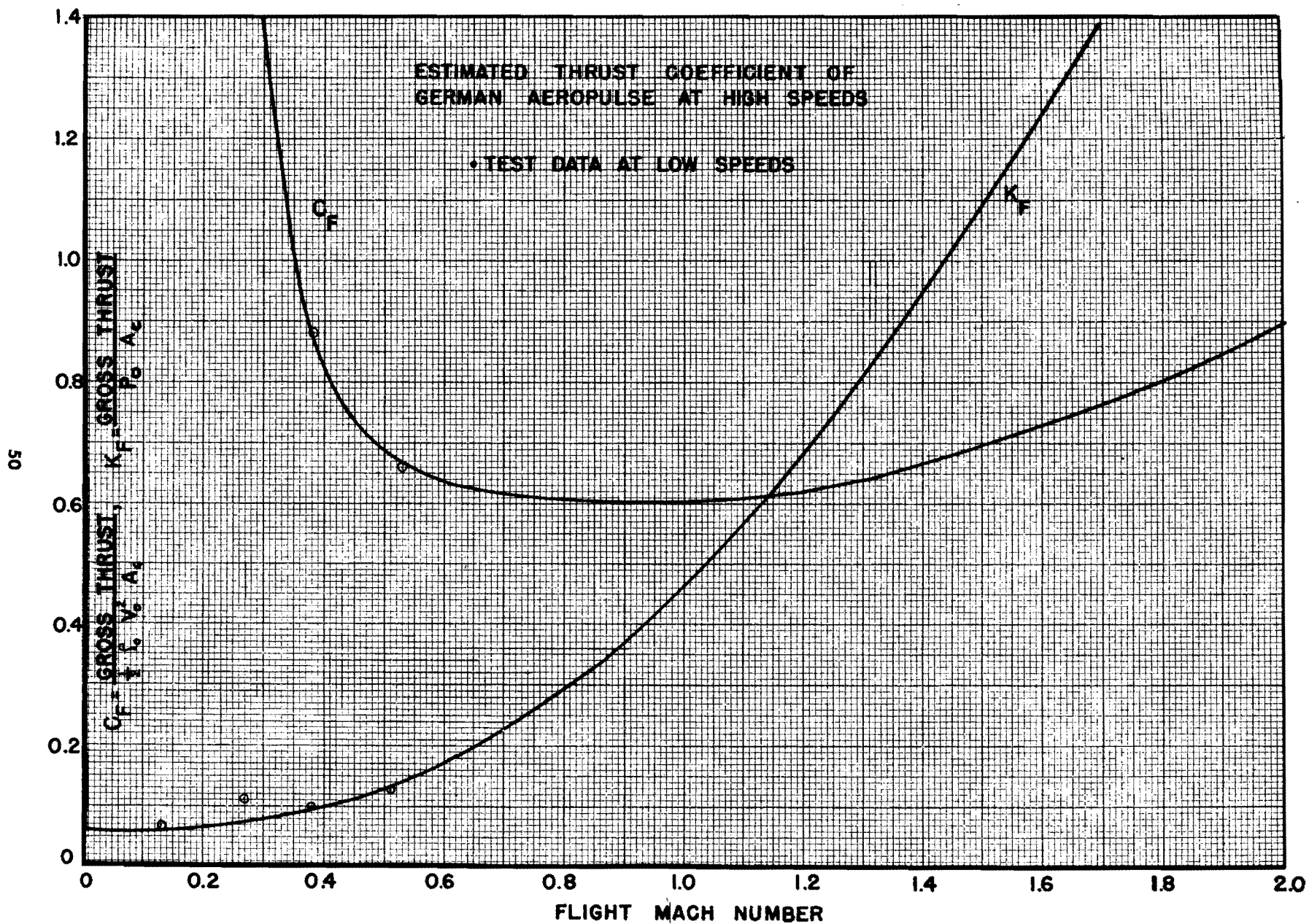
Figure 6 — Estimated Thrust Coefficient of German Aeropulse at High Speeds Test Data at Low Speeds
