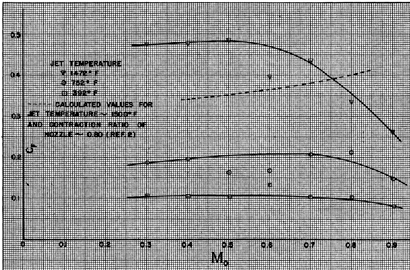
Figure 7 — Calculated Values for Jet Temperature — 1500° F and Contraction Ratio of Nozzle — 0.80 (Ref. 2)
