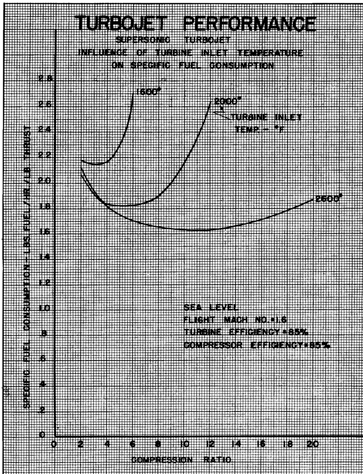
Figure 15 — Turbojet Performance (Supersonic Turbojet Influence of Turbine-Inlet Temperature on Specific Fuel Consumption)
