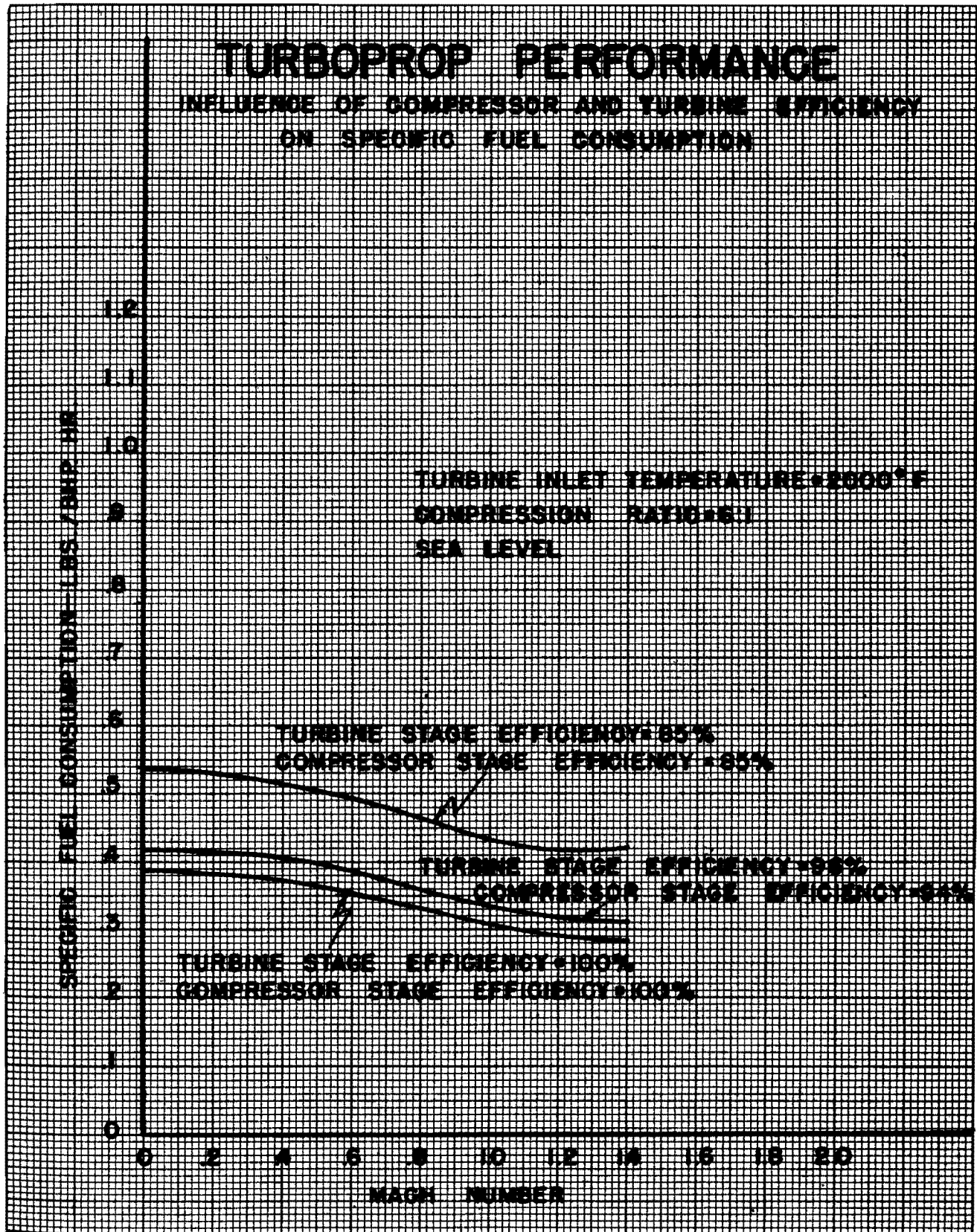
Figure 5 — Turboprop Performance (Influence of Compressor and Turbine Efficiency on Specific Fuel Consumption)
