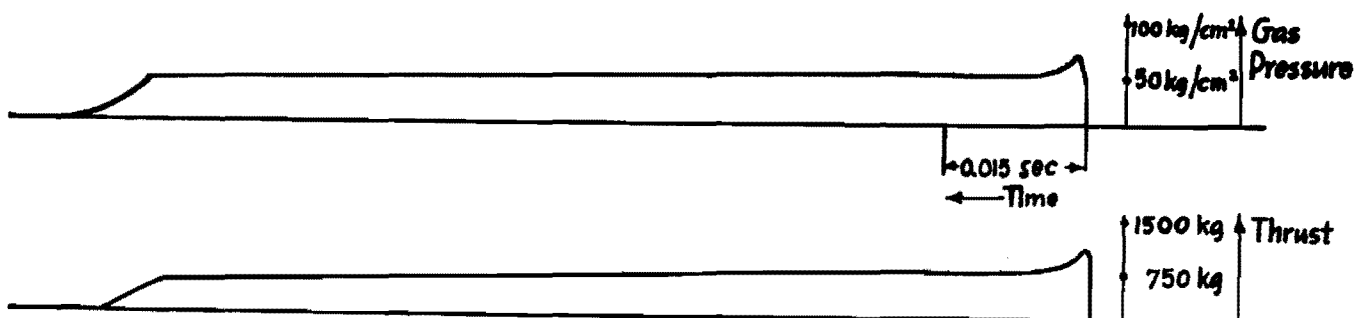
Figure 5 — Smooth Burning
