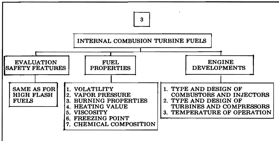
Figure 10 — (Sheet 2) Post War Aviation Fuels — Items Suggested for Discussion
