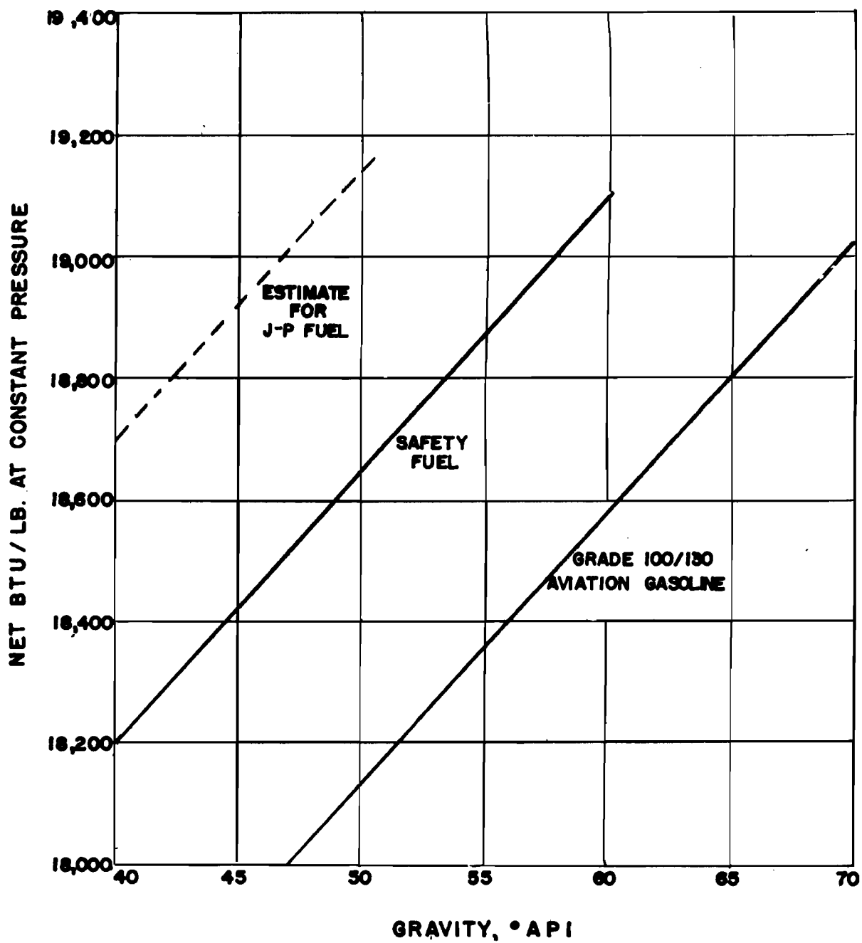
Figure 2 — Chart for Estimating Heating Value from Gravity
