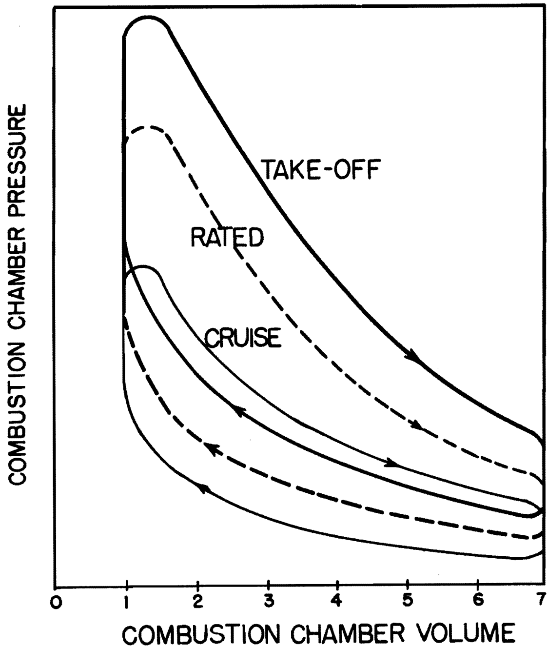
Figure 7 — Pressure-Volume Relationship
