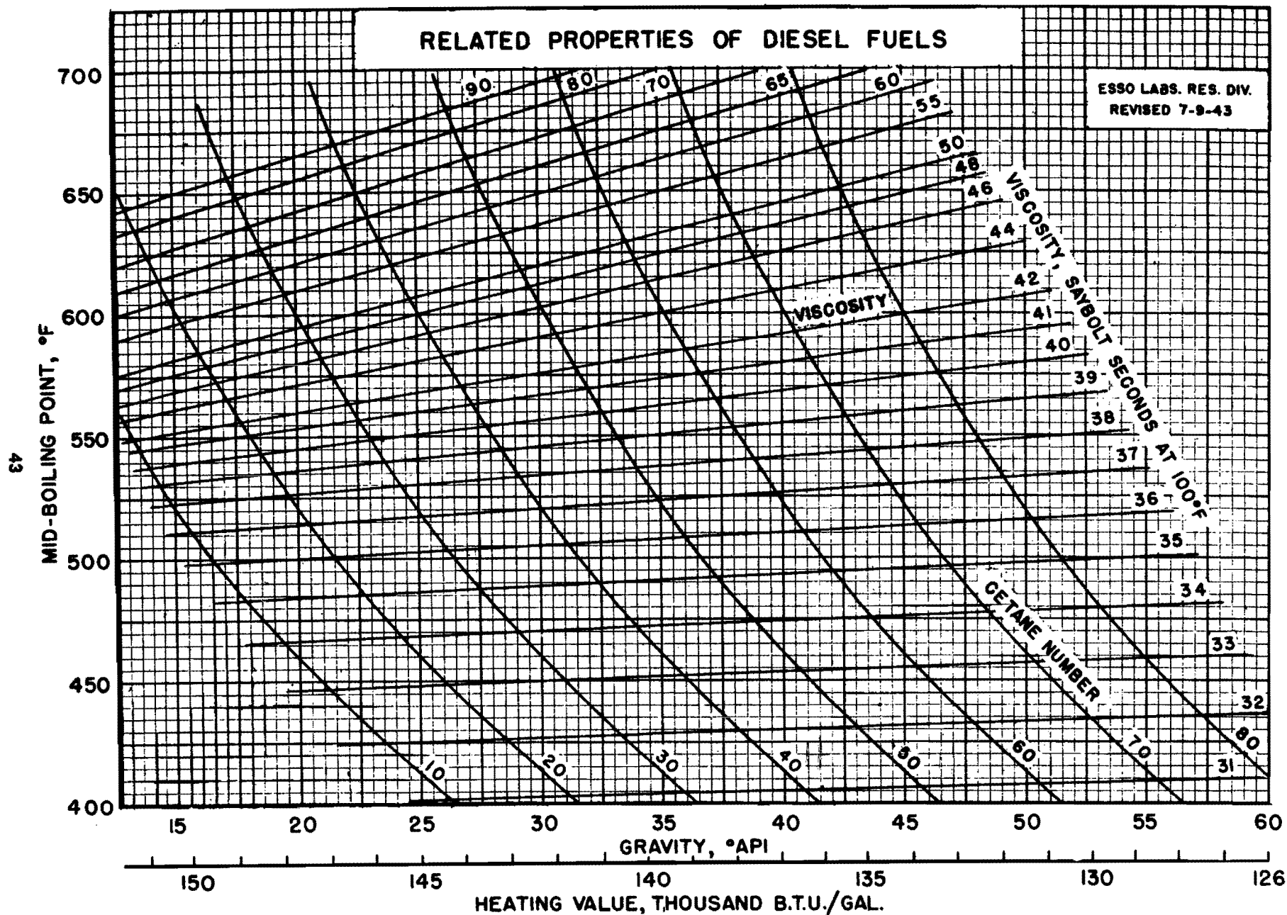
Figure 9 — Related properties of Diesel Fuels
