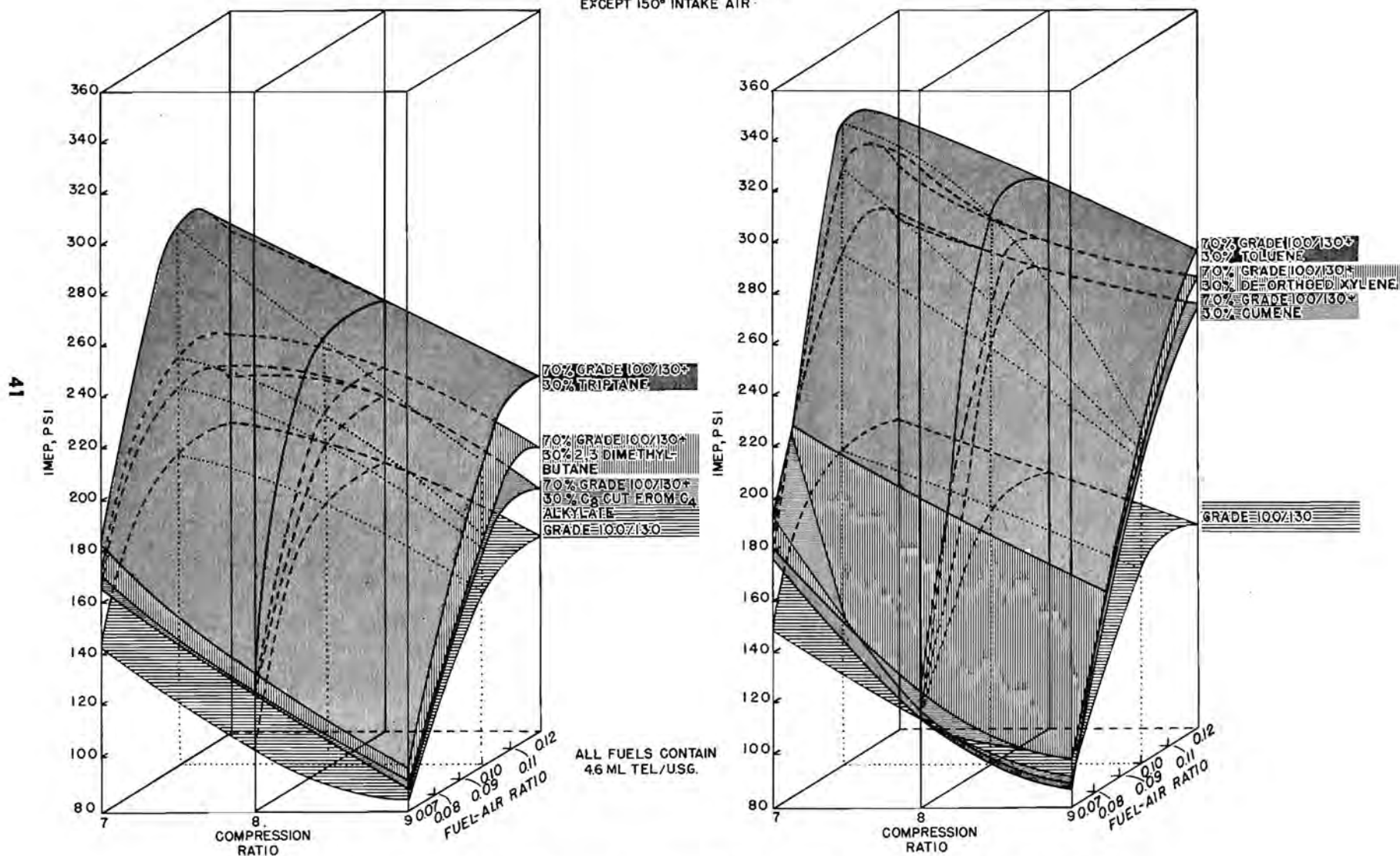
Plate 6 — Effect of Compression ratio and mixture strength on permissible Power Outfit
