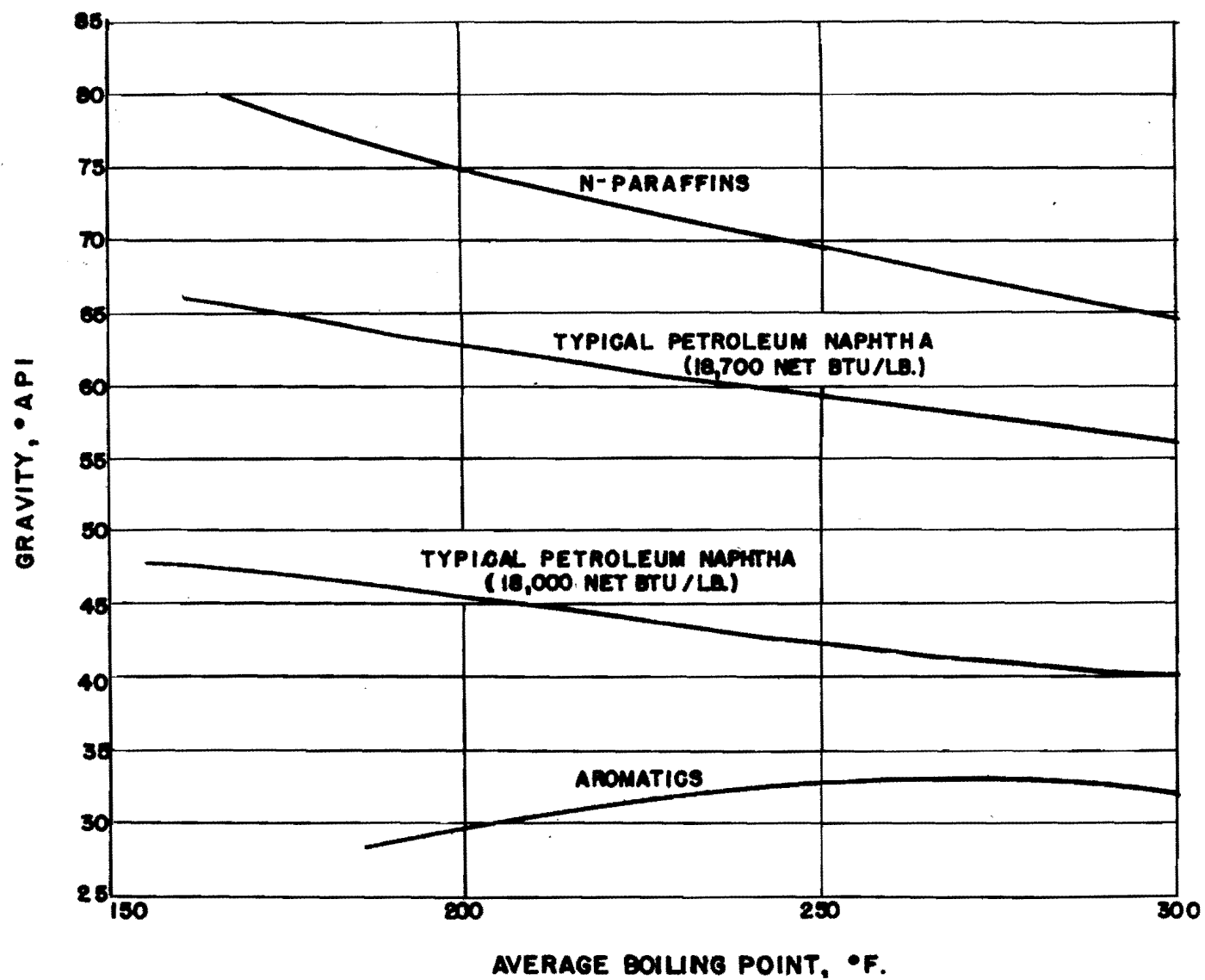
Figure 1 — Trends of Density of Hydrocarbons vs. Boiling Point
