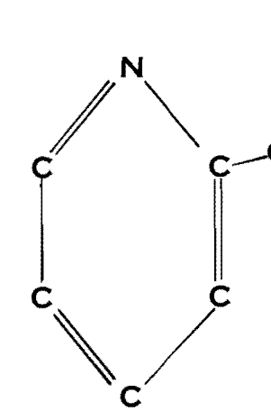
Alpha-PICOLINE
