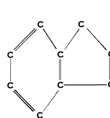
BENZOCYCLOPENTADIENE
