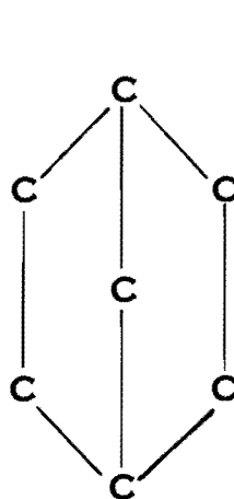
BICYCLO(2,2,1)HEPTANE
