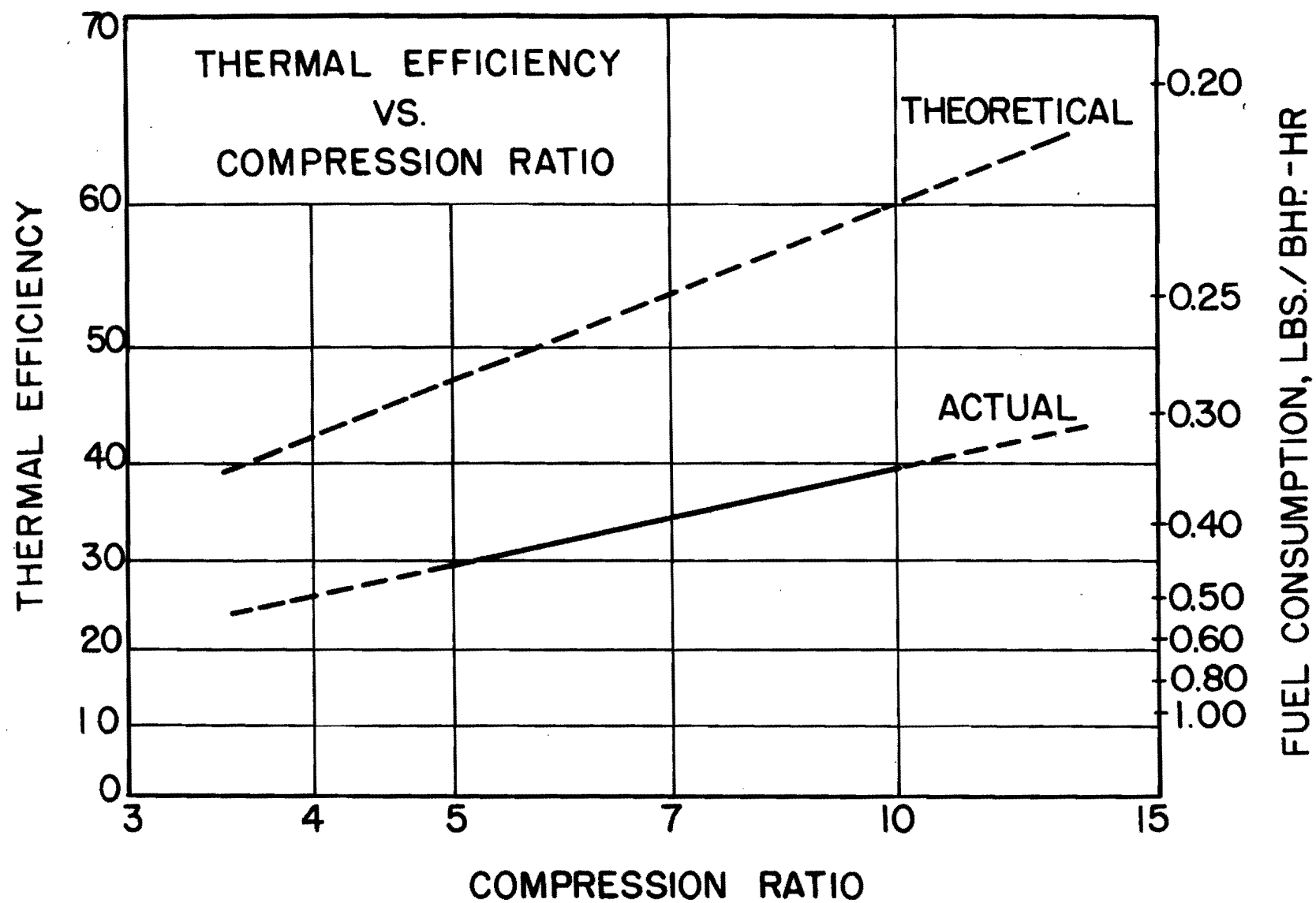
Figure 6 — Thermal Efficiency vs. Compression Ratio
