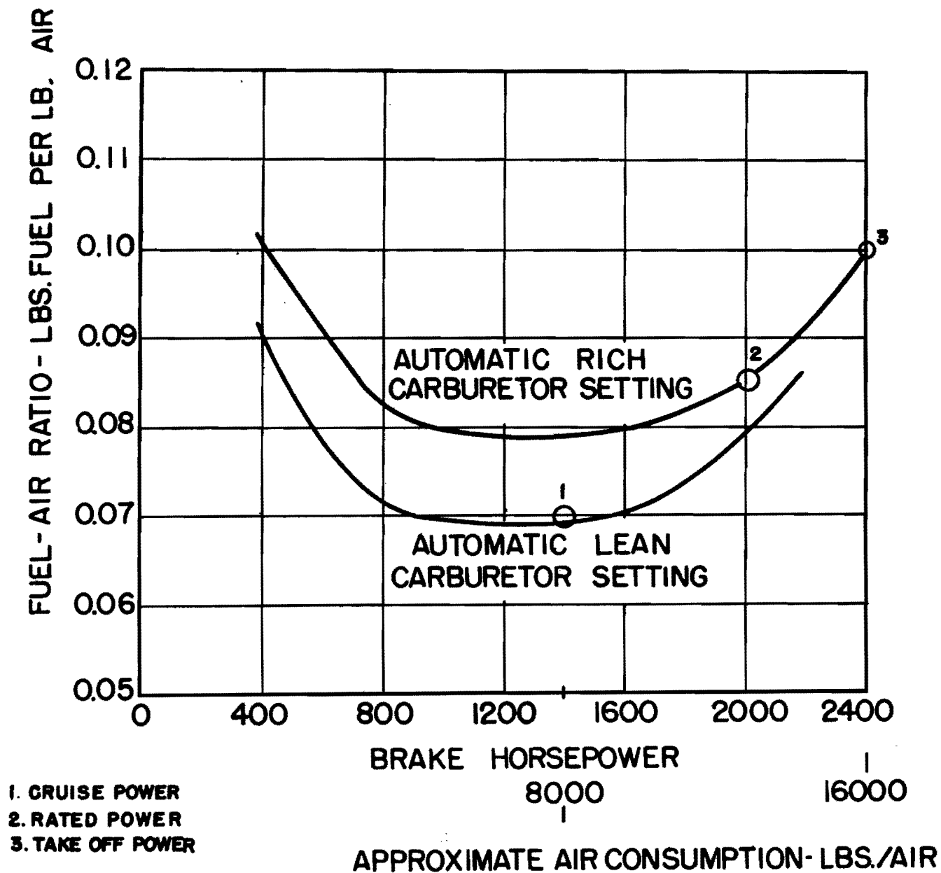
Figure 8 — Typical Mixture Curves
