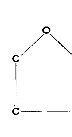
FURAN
