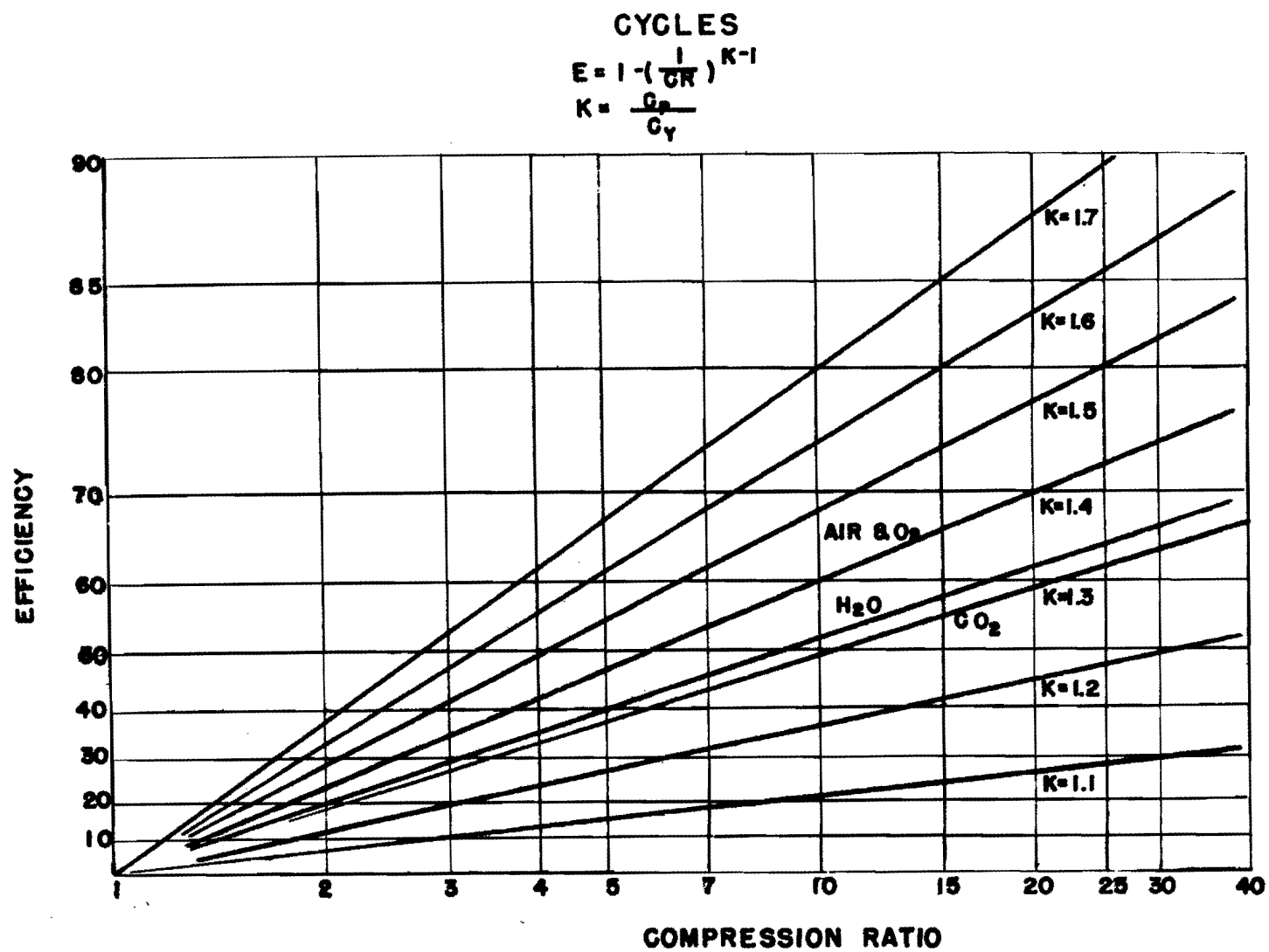
Figure 4—Efficiency vs. Compression Ratio Constant Volume and Constant Pressure
