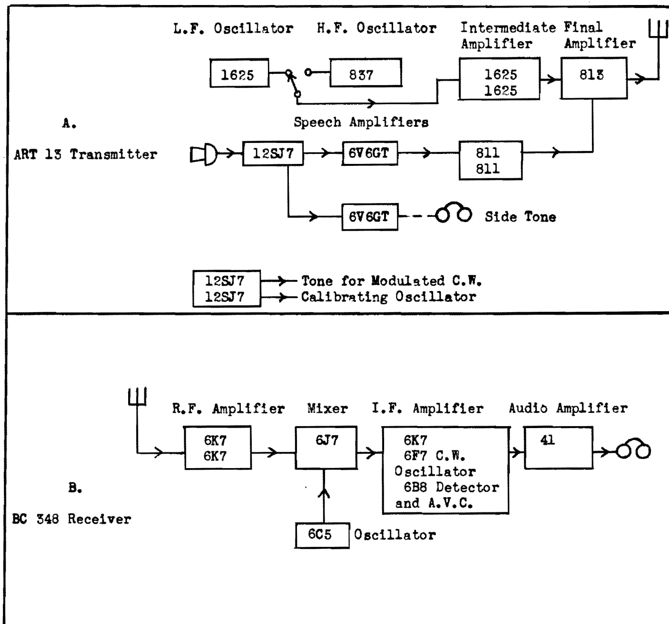
Figure 1 — Block Diagrams of Equipment
