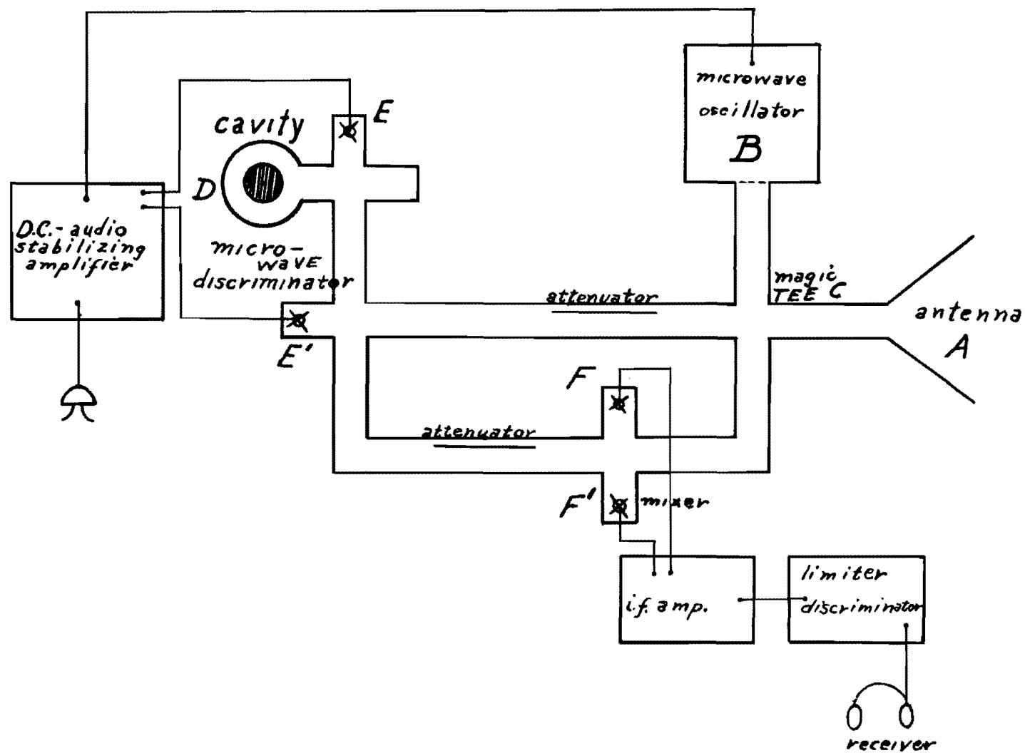
Figure 8 — Stabilized Microwave System
