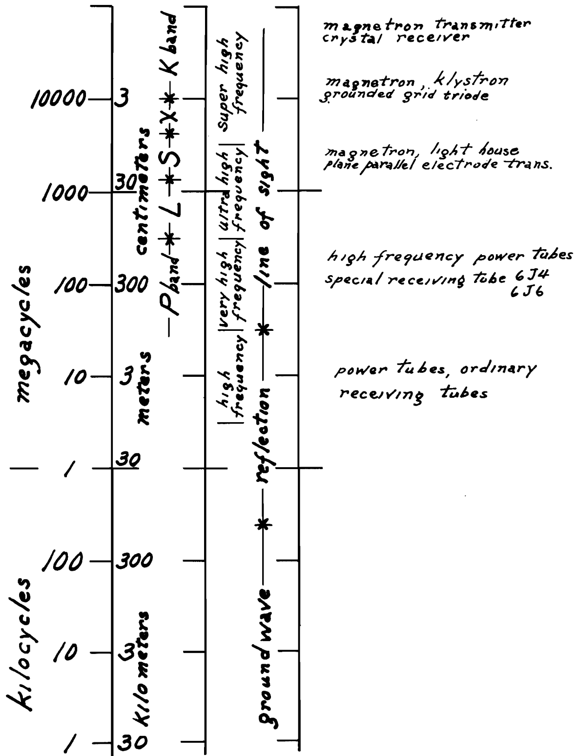
Figure 7 — Radio Spectrum
