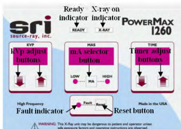
Figure 8. Control Panel Descriptions.
